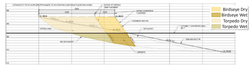
Cross Section of Swimming Cove
