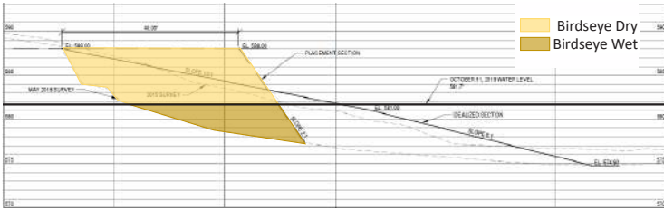
Cross Section of Nature Cove
